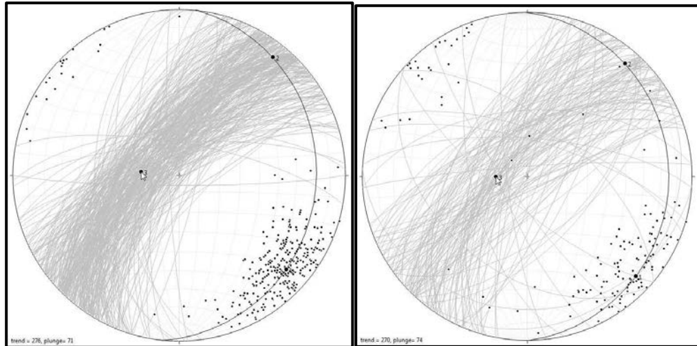
Figure 7.23 Silica Hill Stereonets
