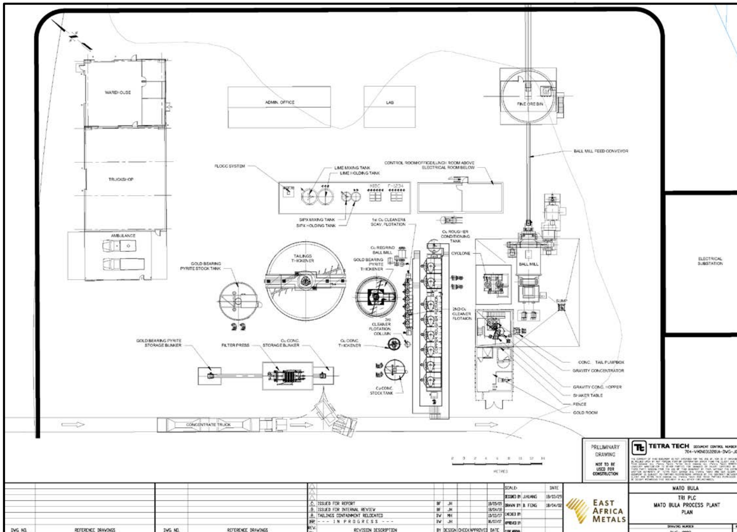
Figure 18.3 Mato Bula Conceptual Plant Site Layout
