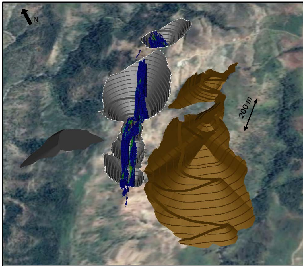
Figure 16.8 Planned WRSF for Open Pit Mining at Mato Bula
